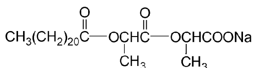
Formula 2: Chemical Structure of Sodium Behenoyl Lactylate
