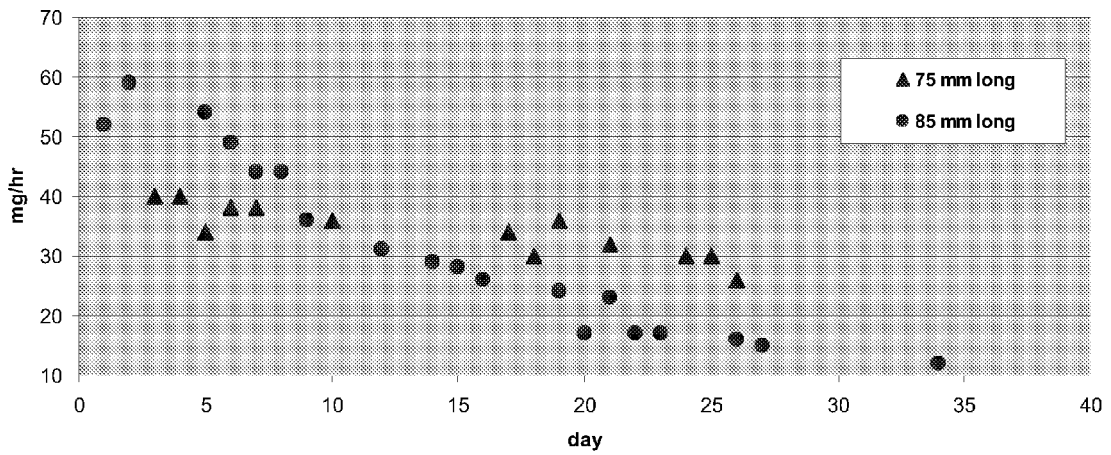
Effect of Wick Length on Wick Blocking 73 micron Porous Plastic, Toggled
