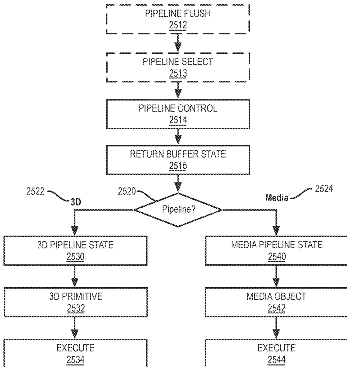
FIG. 25B GRAPHICS PROCESSOR COMMAND SEQUENCE 2510
