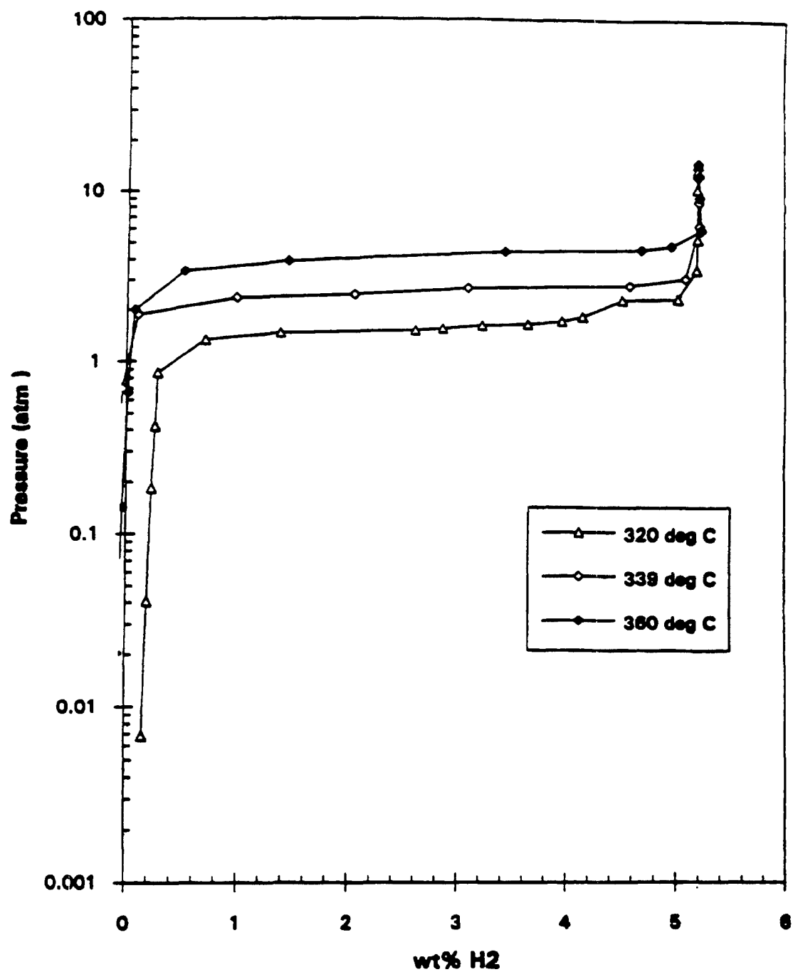
Figure 9 P-C Isotherms of a Mg-Ni-Mo system, MA-2
