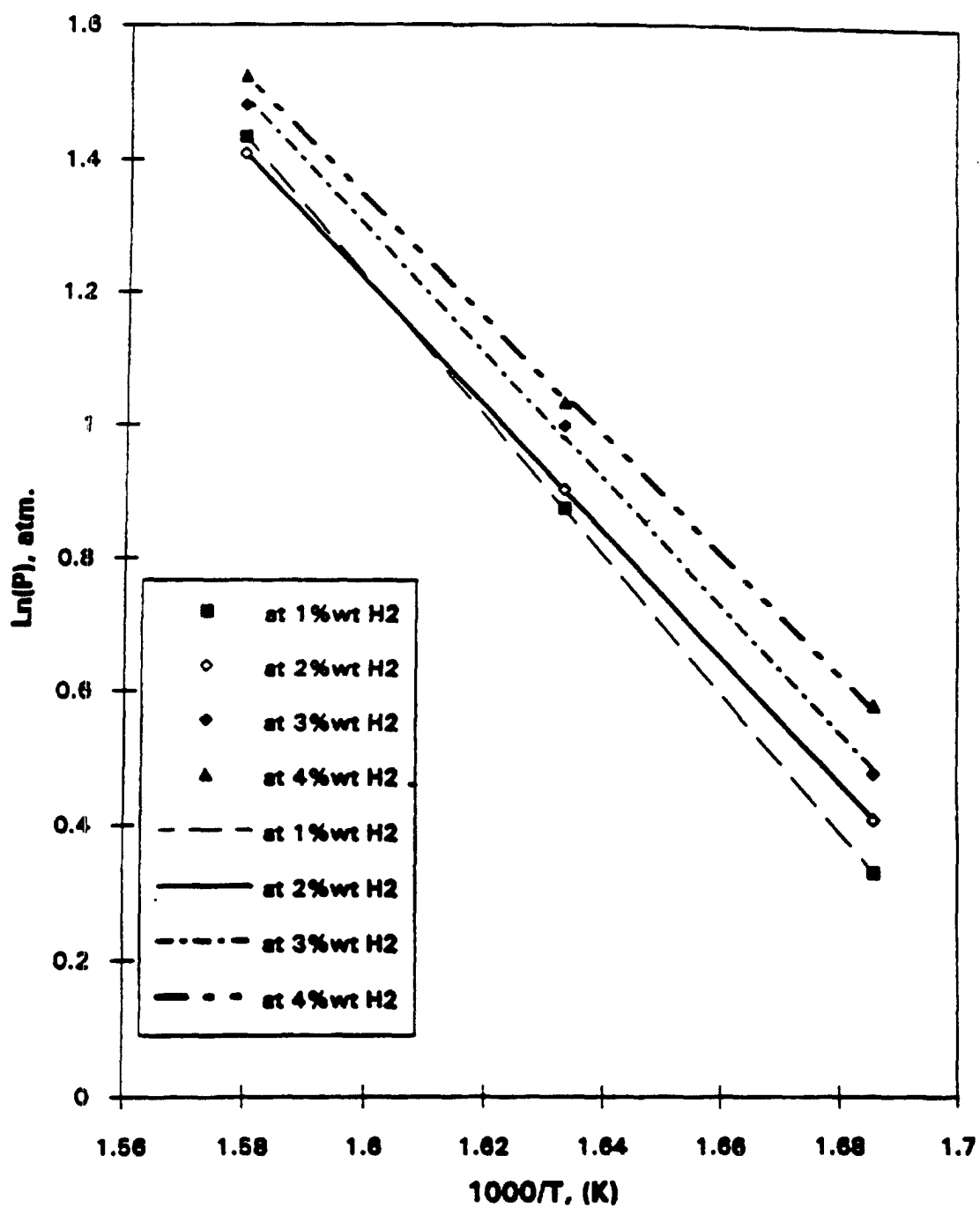
Figure 10 Van't Hoff Plot for Desorption of MA-2
