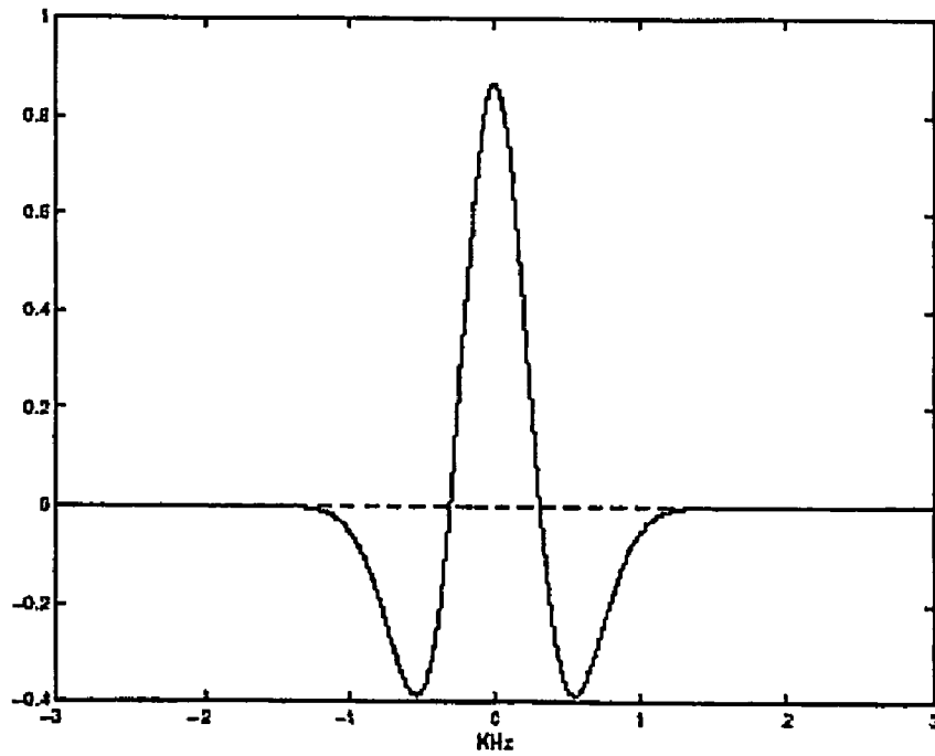
FIGURE 8(b) Transverse magnetization profile.
