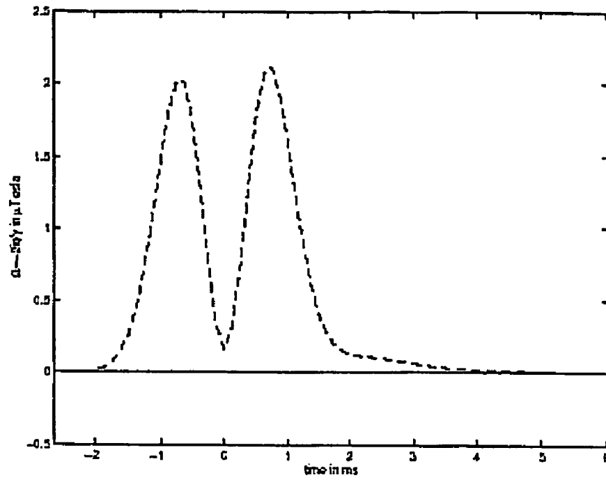
FIGURE 8 (a) Minimum energy pulse.
