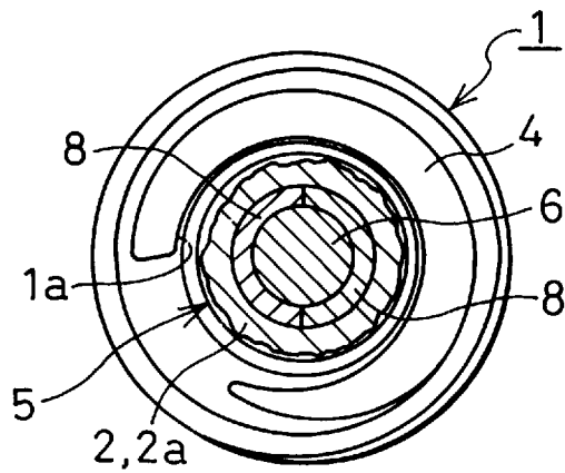
FIG. 4 PRIOR ART
