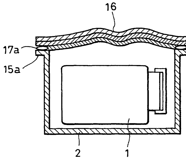
FIG. 6 PRIOR ART
