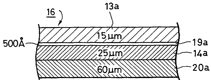
FIG. 7 PRIOR ART
