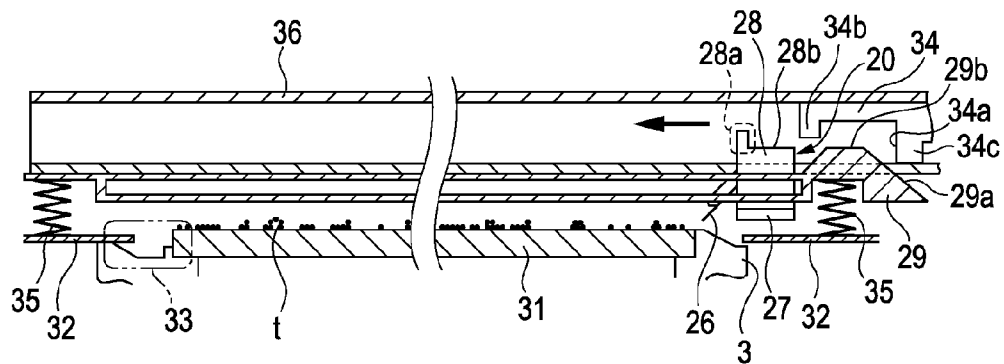
FIG. 5A HOME POSITION
