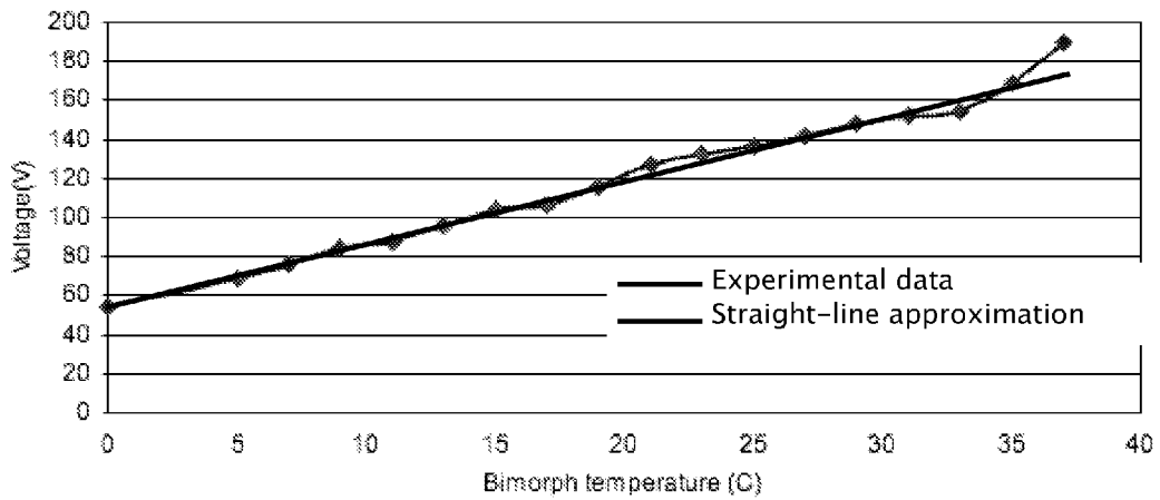
Lift-off voltage Vs Temperature
