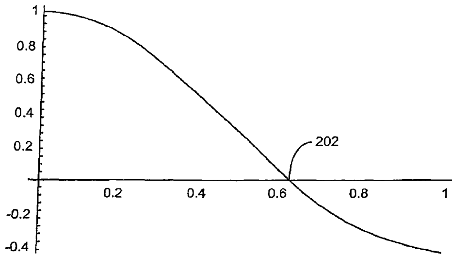
Radial Distribution of U for the (0,1) mode
