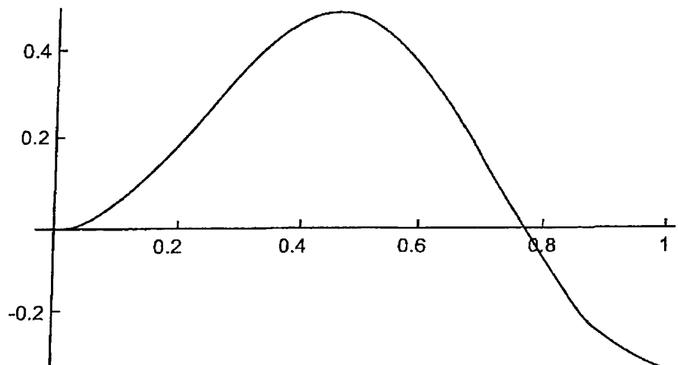
Radial Distribution of U for the (2,2) mode
