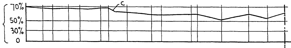
FIG. 7(b) BATTERY BANK STATE OF CHARGE (BSC)
