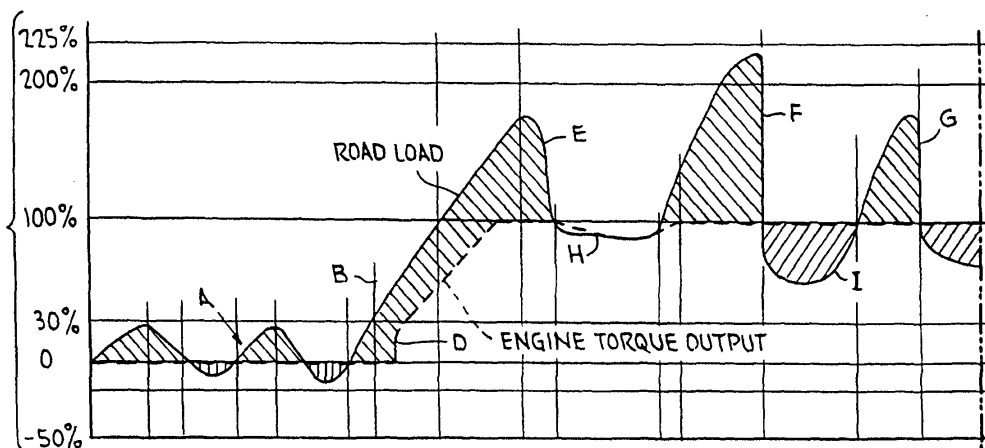
FIG. 7(a) ROAD LOAD AS% OF MAX. ENGINE TORQUE OUTPUT (% MTO)
