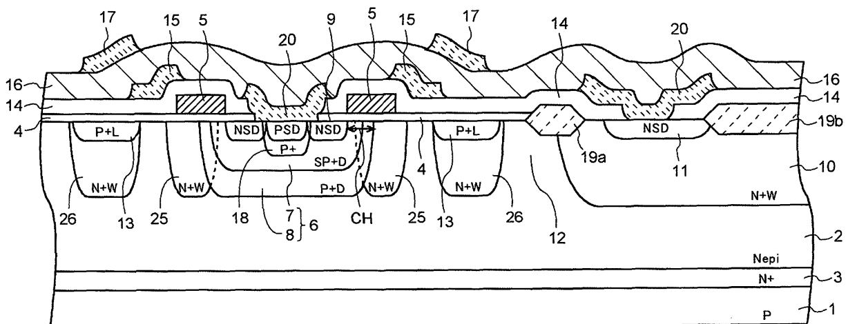
FIG.1 Transistor A
