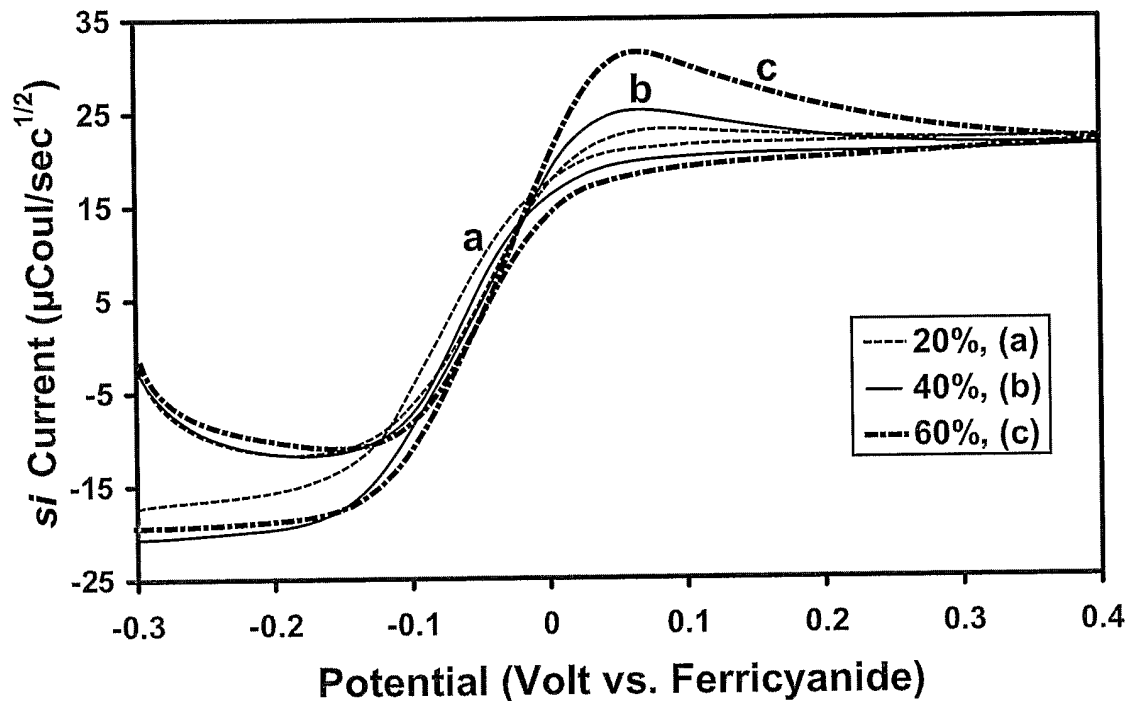
Cyclic Semi-integrals at 50 mg/dL WB, 0.025 V/sec
