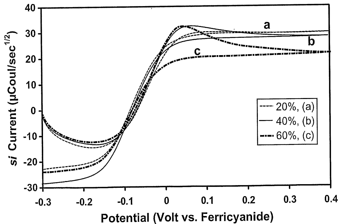
Cyclic Semi-integrals at 100 mg/dL WB, 0.025 V/sec
