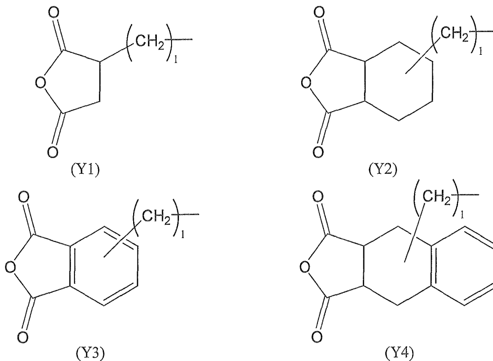
[Chemical Formula 8]
