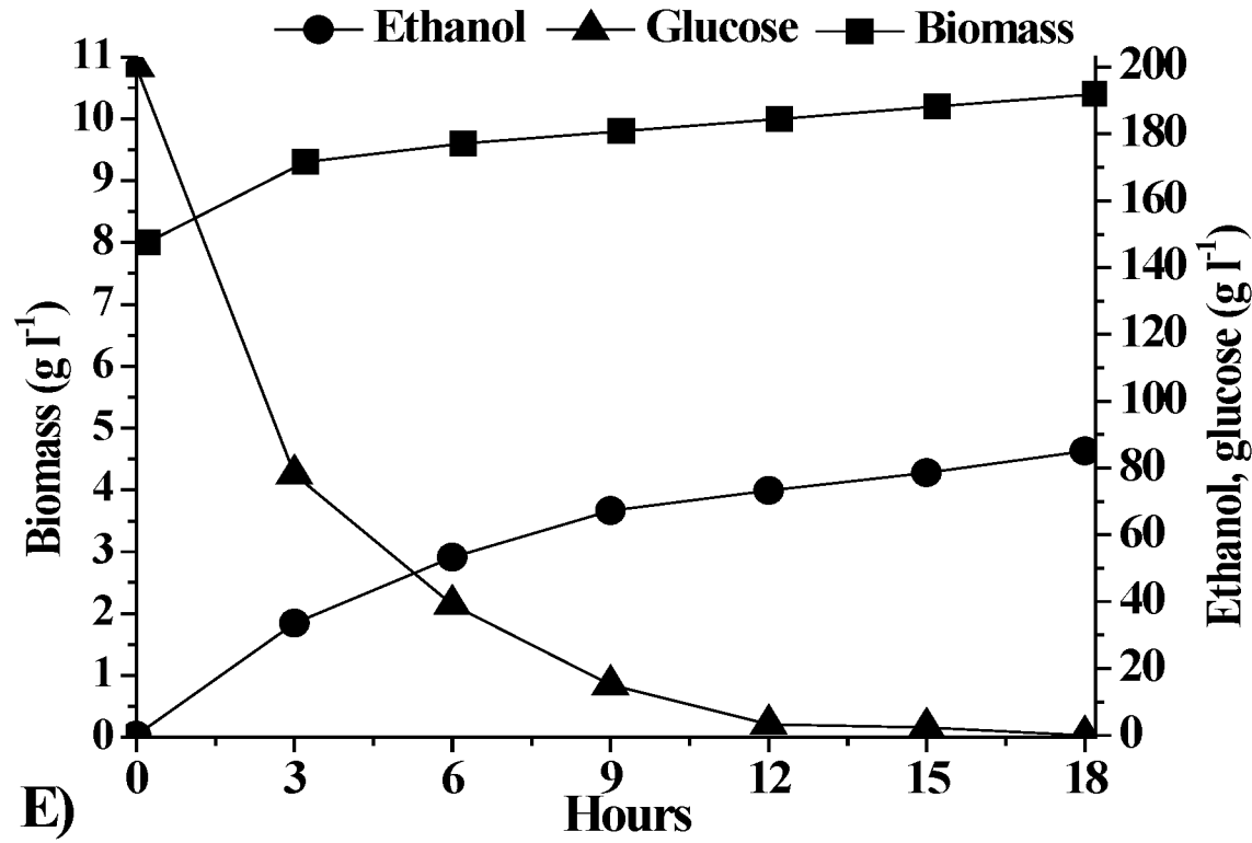
FIG. 5: AS400-510 fermentation
