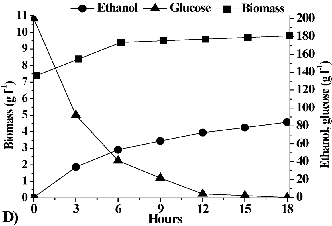
FIG. 4: AS400-617 fermentation
