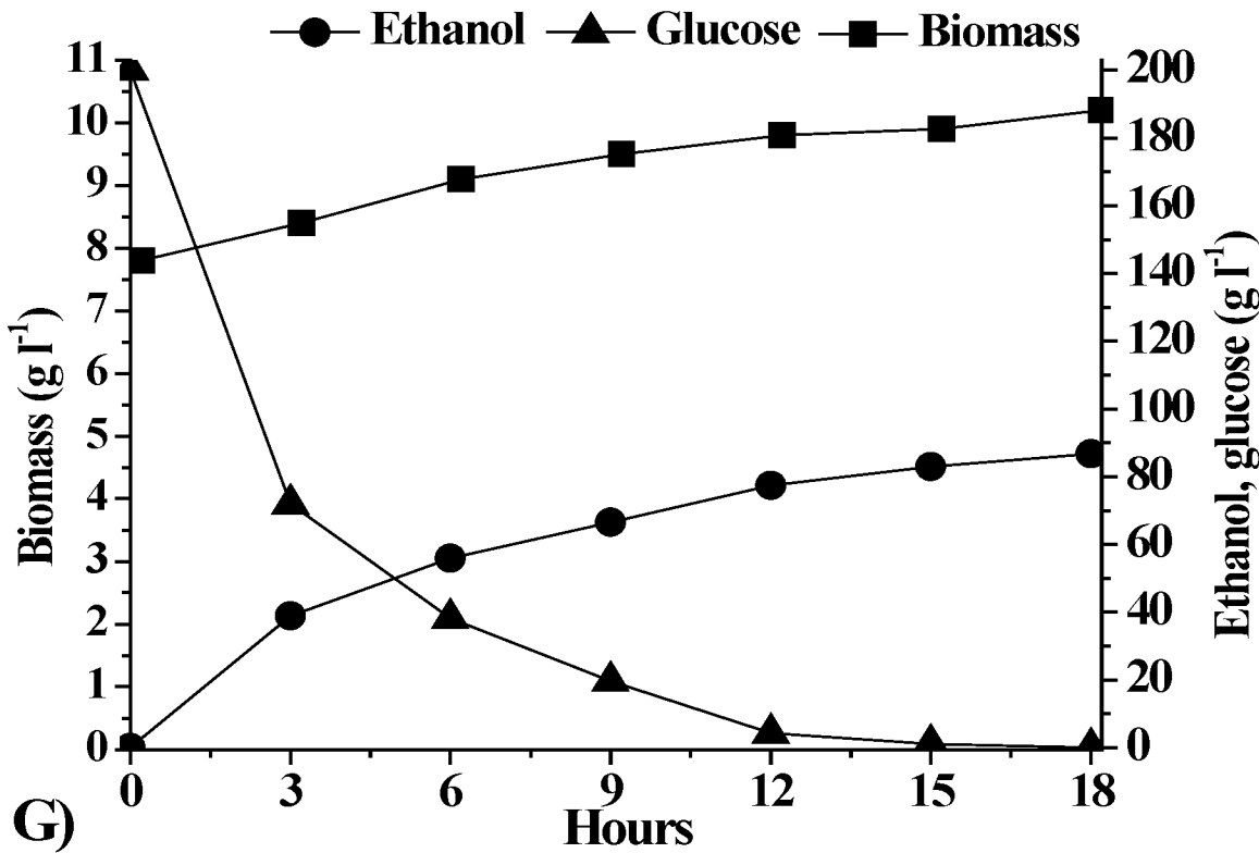
FIG. 7: AS400-510-42 fermentation
