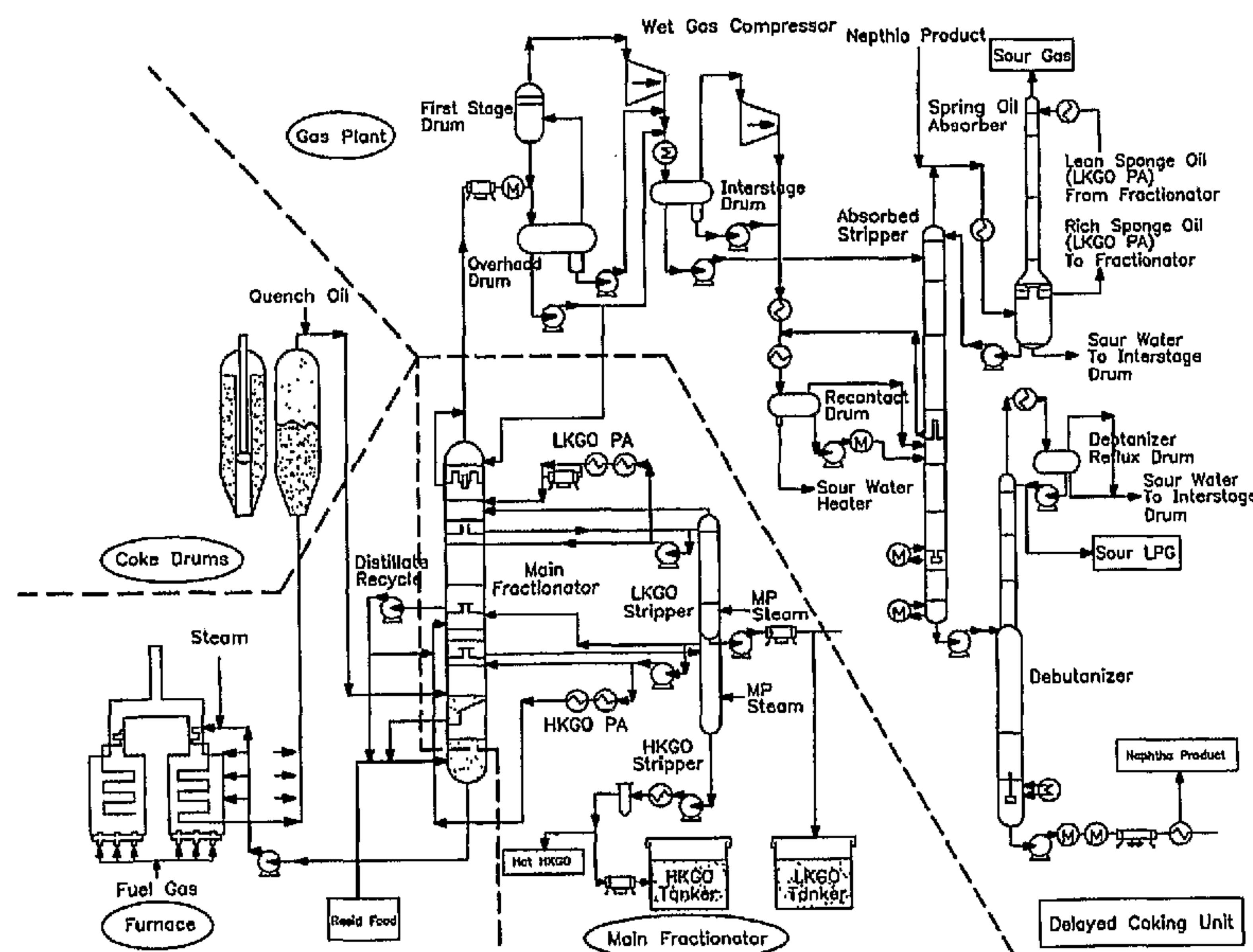
DCU and Light Ends Processing Units
