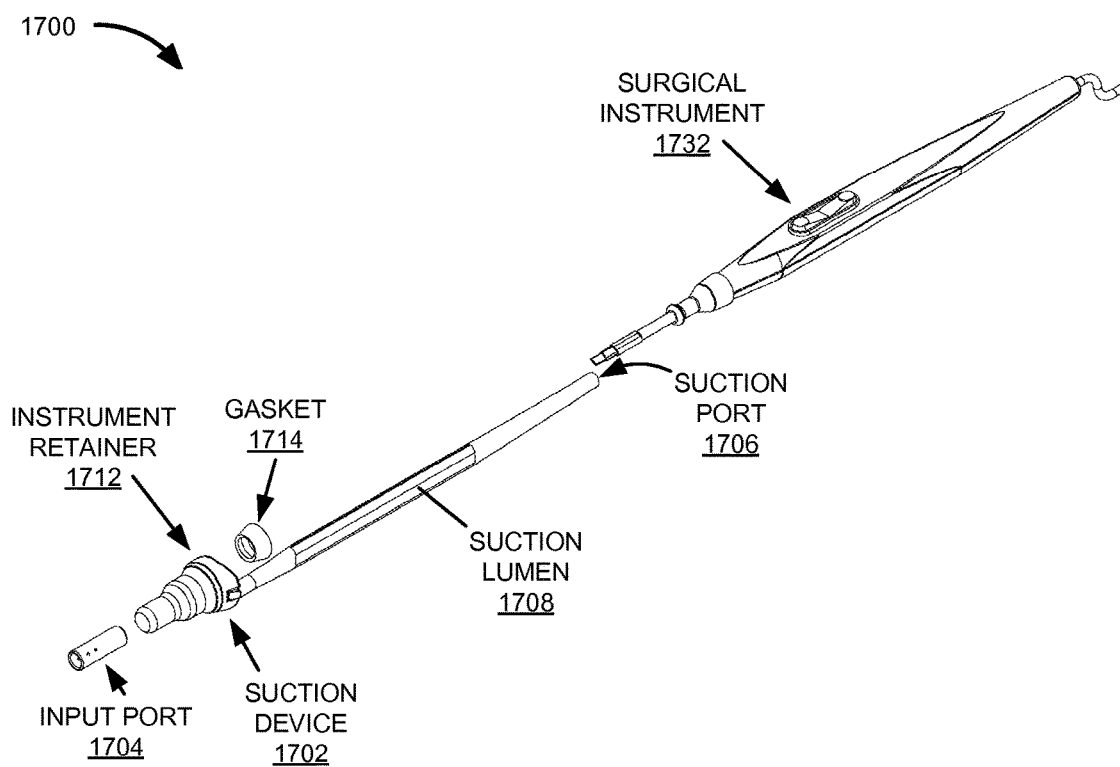
FIGURE 17B
