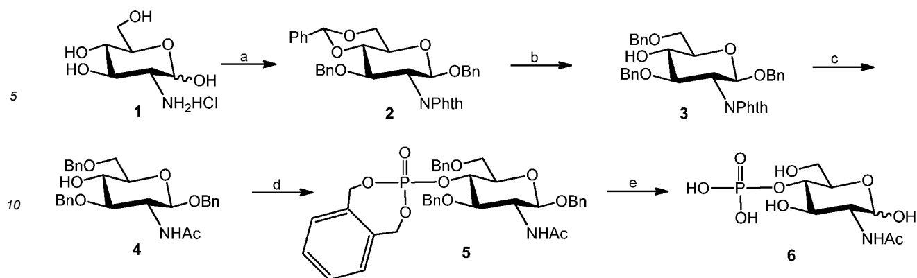
Scheme 1. a. Ref. 236; b. trimethylamineborane, \text{BF}_3 \cdot \text{Et}_2\text{O} , \text{CH}_3\text{CN} , 0^\circ\text{C} , 83%; c. \text{H}_2\text{NCH}_2\text{CH}_2\text{NH}_2 , \text{EtOH} , reflux; \text{Ac}_2\text{O} , pyridine, 87% (over 2 steps); d. N,N -diethyl-1,5-dihydro-3 H -2,3,4-benzodioxaphosphin-3-amine, 1 H -tetrazole, \text{CH}_2\text{Cl}_2 ; m -CPBA, \text{CH}_2\text{Cl}_2 , \text{H}_2\text{O} , 92%; e. \text{H}_2 , 10% Pd-C, 95%.
