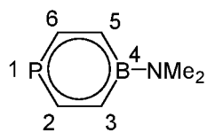
4-dimethylamino- 1,4-phosphaboratabenzene
