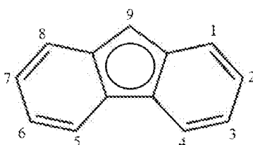
Fluorenyl
