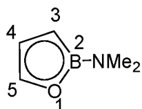
2-dimethylamino- 1,2-oxaborollide
