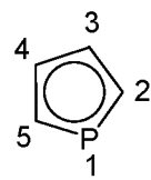
phosphacyclopentadienyl
