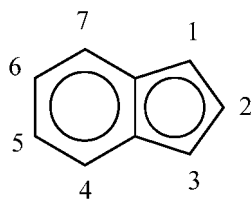
Indenyl
