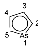
arsacyclopentadienyl
