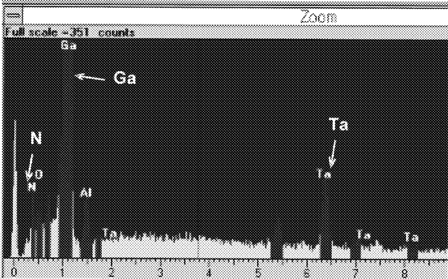
(B) EDX spectrum
