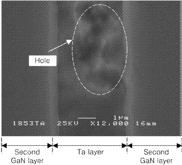
(B) SEM micrograph of surface of substrate
