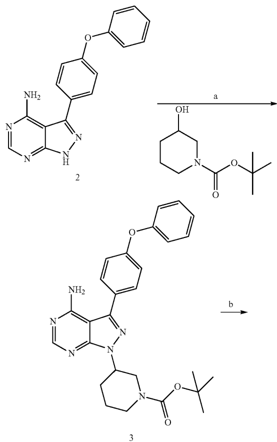
Scheme 1. Synthesis of compound 4;
