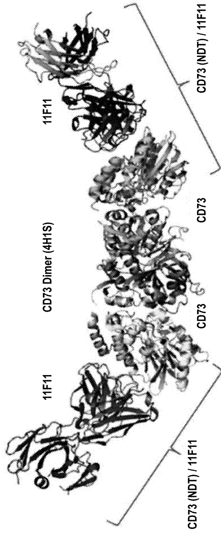
Composite structure of two CD73(NDT)/11F11 complexes superimposed on CD73 dimer (PDP Entry 4H1S)
