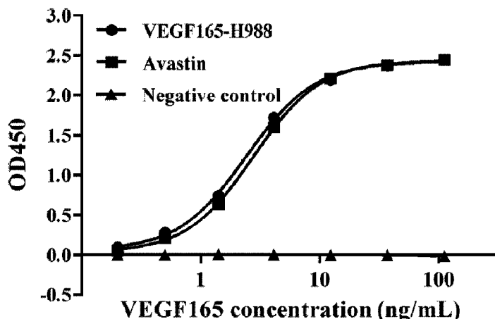
The ELISA assay result of the binding of humanized antibody VEGF165-H988 to VEGF165
