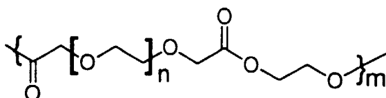
POLY"OXA"ESTERS
