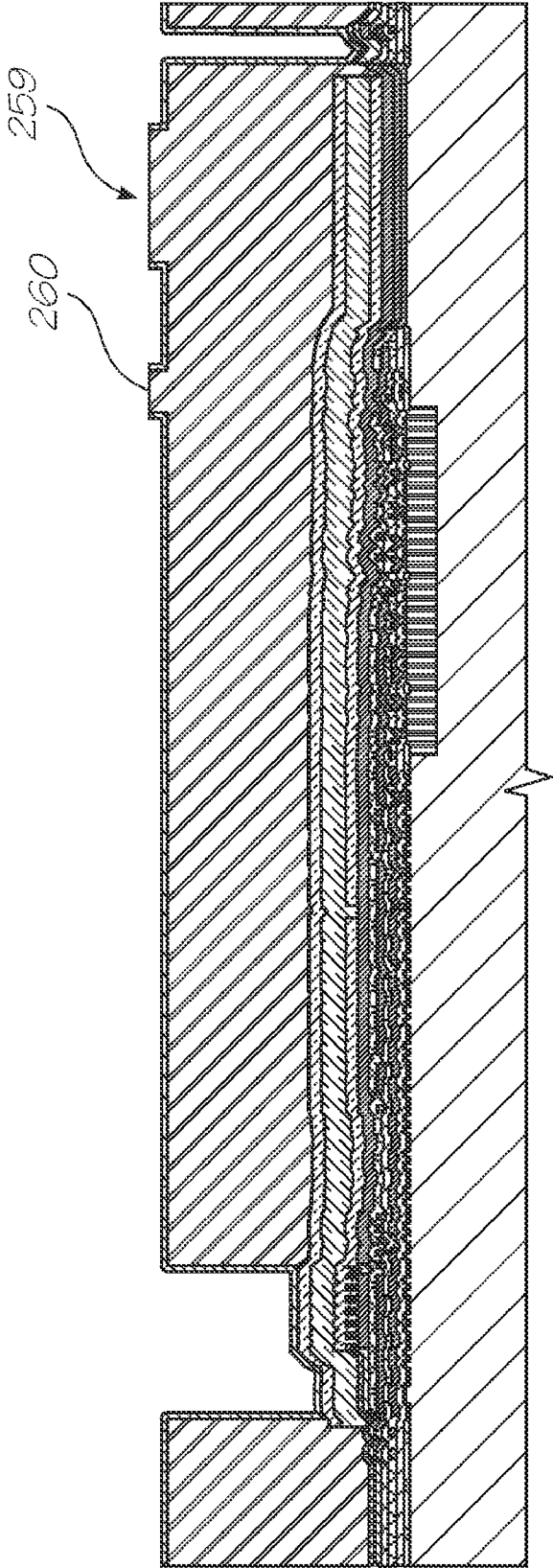
Form self-aligned nozzles using CMP
