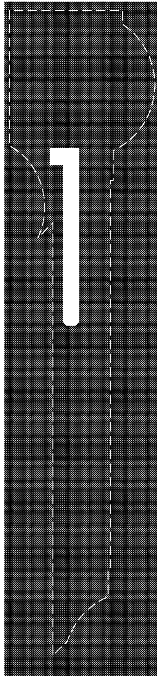
N-Well mask
