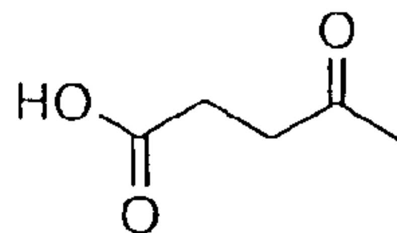
levulinic acid
