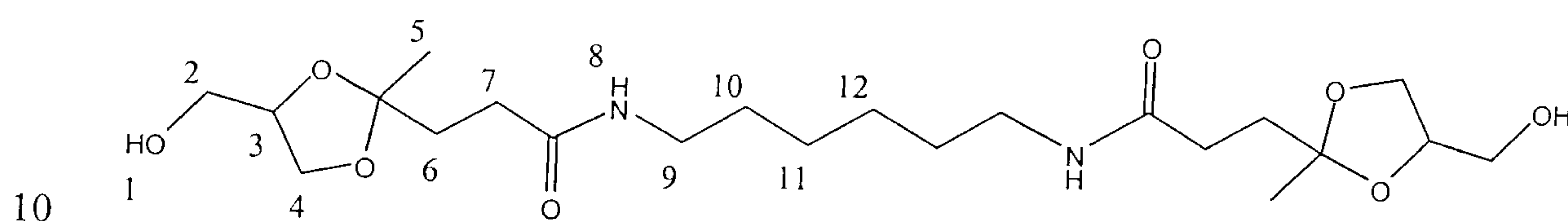
Proton assignments
