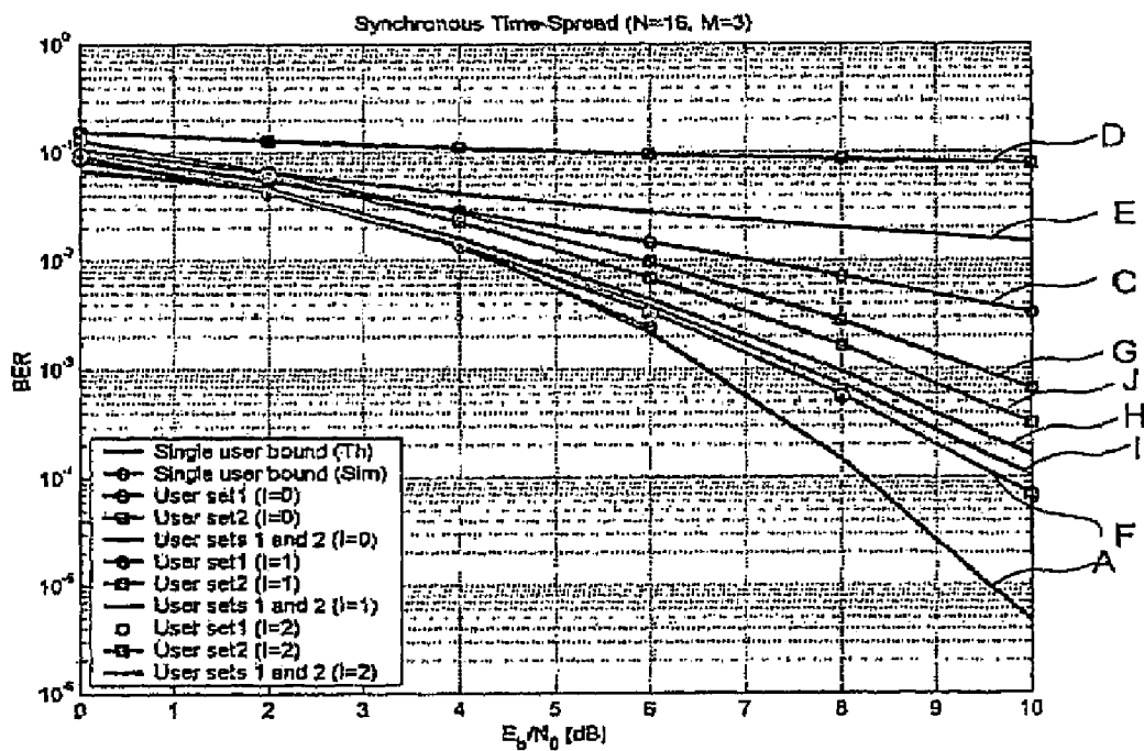
Simulation results with N=16, M=3
