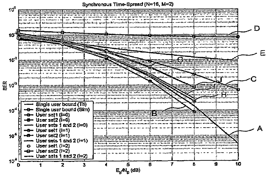
Simulation results with N=16, M=2
