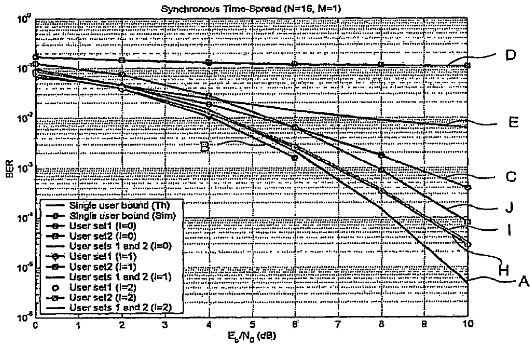
Simulation results with N=16, M=1
