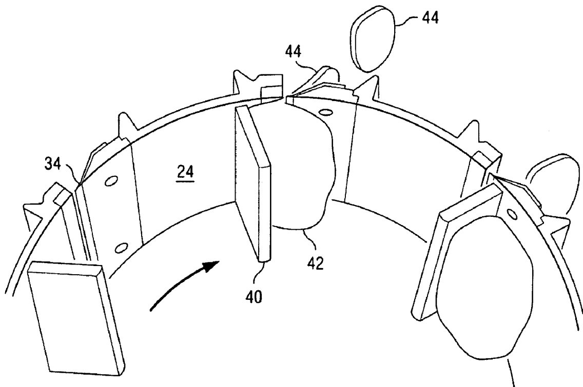
FIG. 4 (PRIOR ART)
