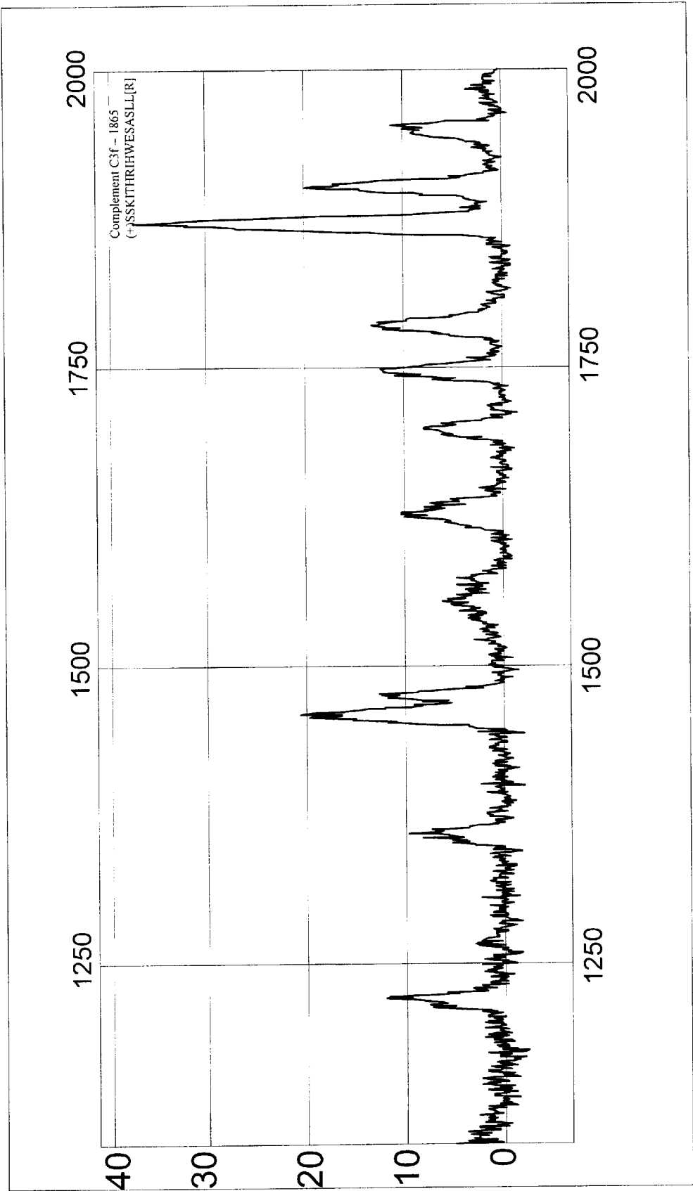
SPECTRA SHOWING DISEASE INDICATIVE MARKER FIGURE 2C
