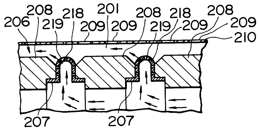
FIG. 5 PRIOR ART
