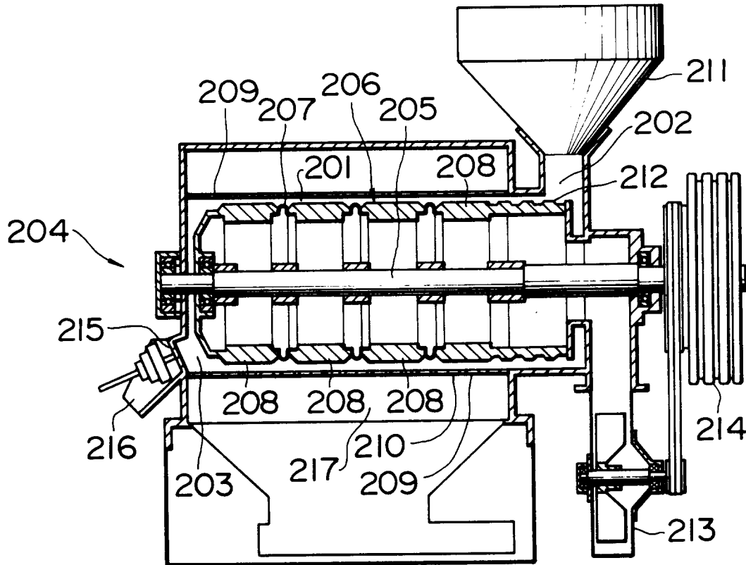
FIG. 4 PRIOR ART
