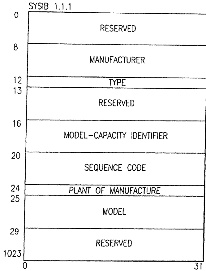
FIG.6 Prior Art
