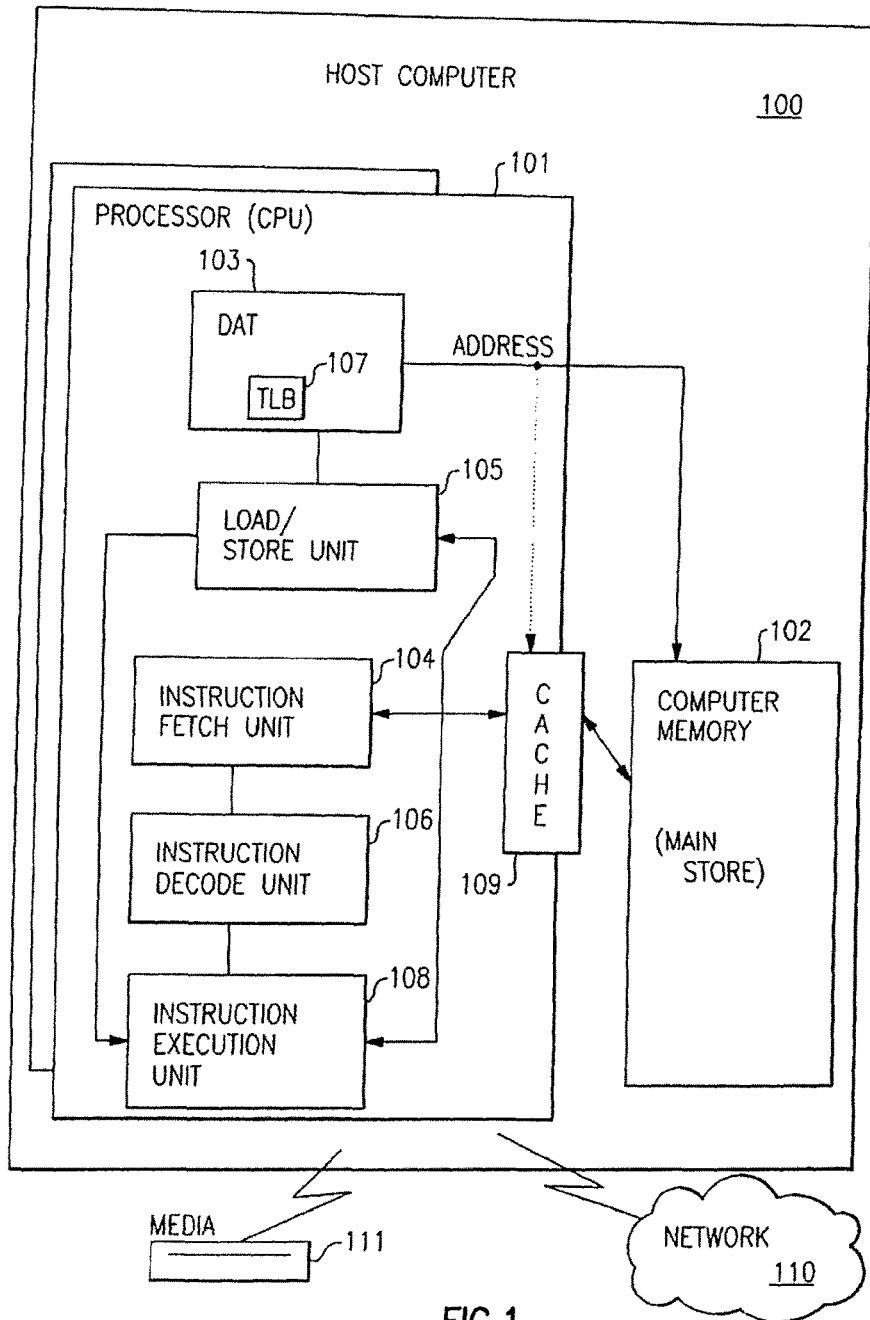
FIG.1 Prior Art
