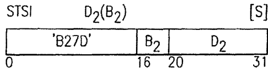
FIG.3 Prior Art
