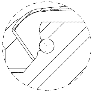
FIG. 9 PRIOR ART
