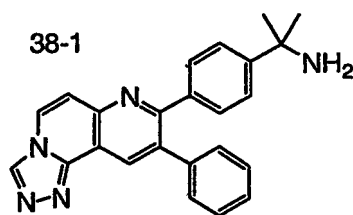
2-[4-(9-phenyl[1,2,4]triazolo[3,4-f]-1,6-naphthyridin-8-yl)phenyl]propan-2-amine ( 38-1 )
