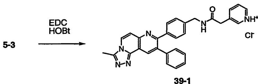
25 3-(2-([4-(3-methyl-9-phenyl[1,2,4]triazolo[3,4-f]-1,6-naphthyridin-8-yl)benzyl]amino)-2-oxoethyl)pyridinium chloride ( 39-1 )
