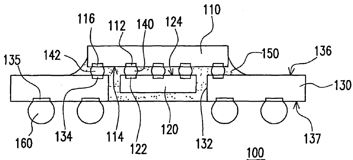
FIG. 1 (PRIOR ART)
