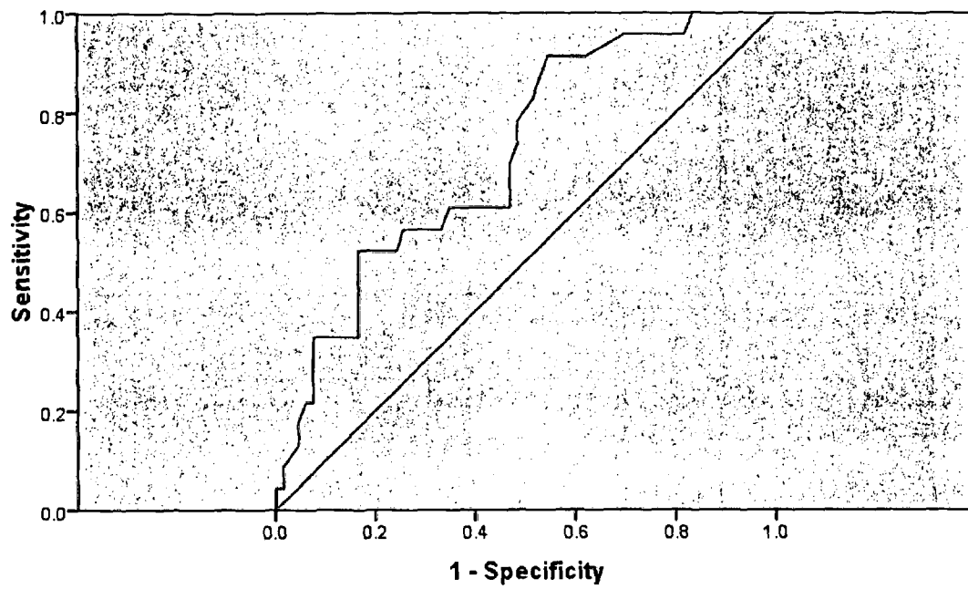
ROC Curve
