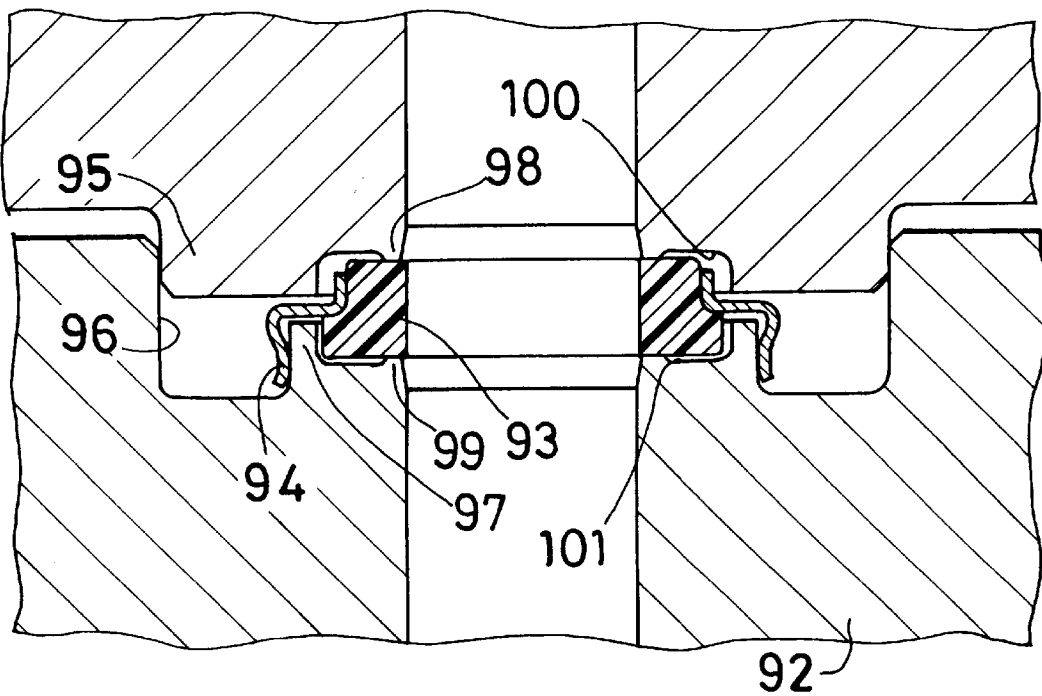
FIG. 10 (PRIOR ART)
