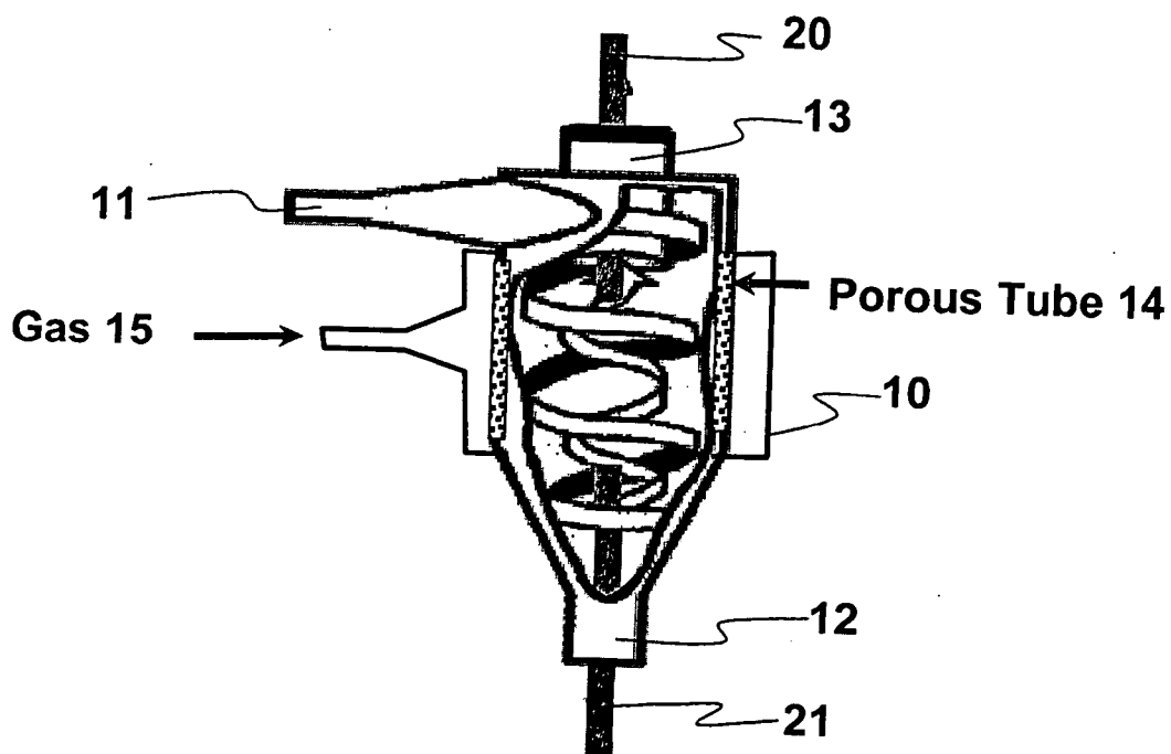
Fig. 3 - Carbon Arc in Gas-Sparged Hydrocyclone
