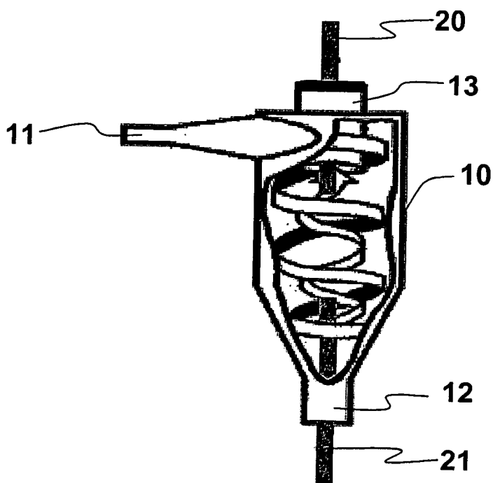
Fig. 2 - Carbon Arc in Cyclone Separator
