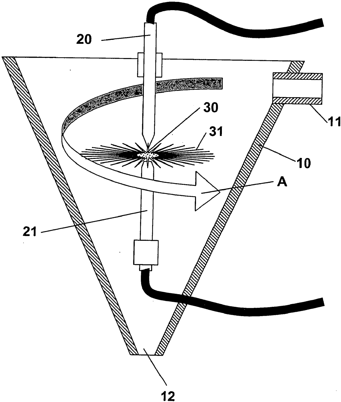
Fig. 1 - Treatment of Fluids With Carbon Arc
