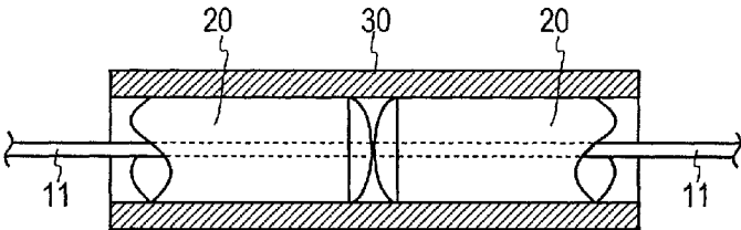
FIG.21 Prior Art
