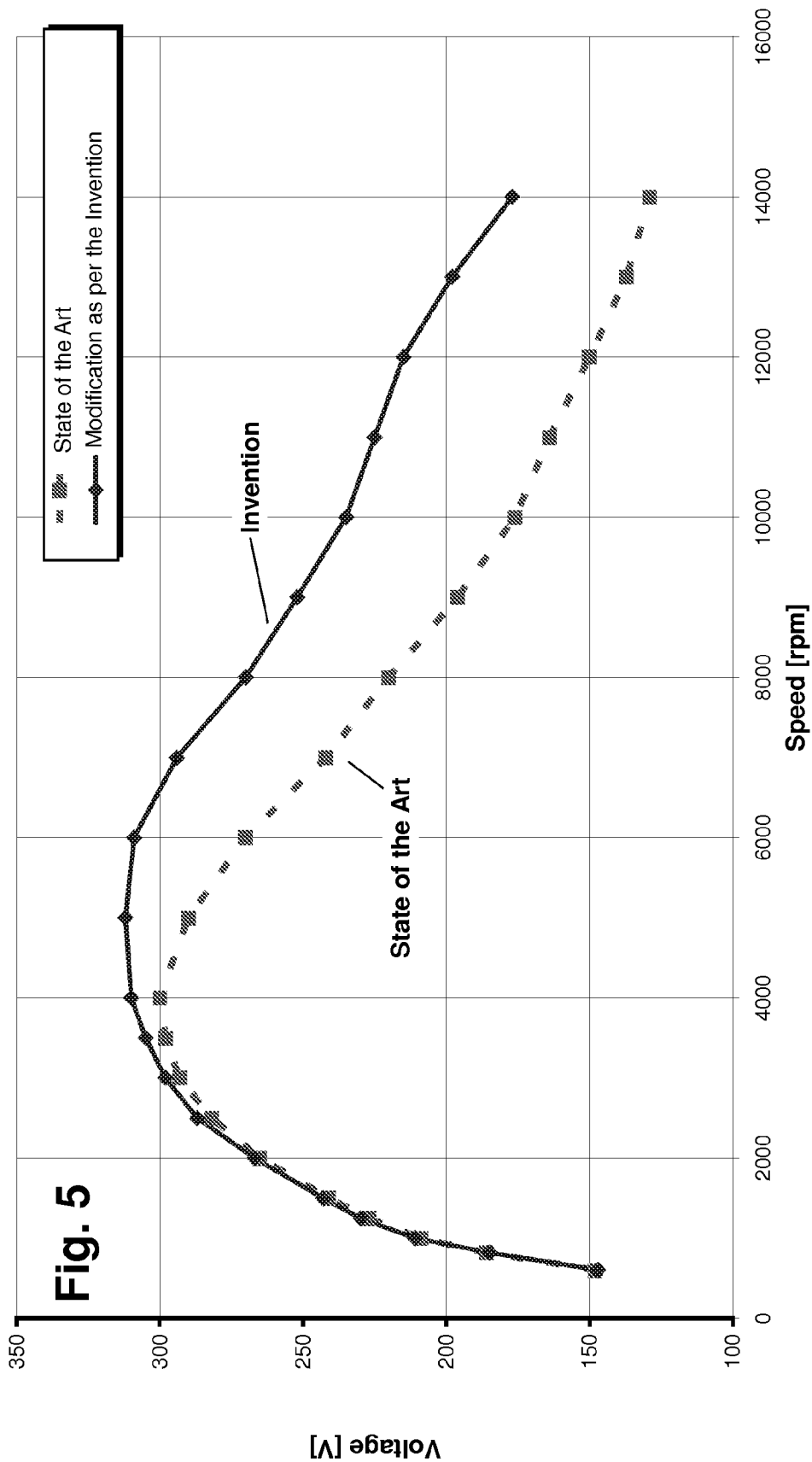
Voltage of Ignition Capacitor Over r.p.m.
