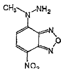
N-methyl-4-hydrazino -7-nitrobenzofurazan
