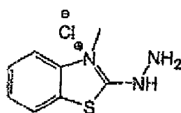
3-methyl-2-benzothiazolinone hydrazone hydrochloride
