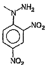
1-methyl-1- (2,4-dinitrophenyl)hydrazine
