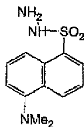
5-(dimethylamino)naphthalene -1-sulphonyl hydrazide
