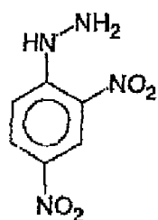
1-(2,4-dinitrophenyl) hydrazine (DNPH)
