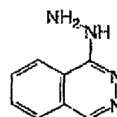
Hydralazine or 1-Hydrazinophthalazine
