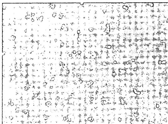
Compound 2
