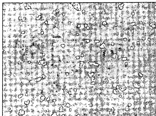
Compound 3 DZNep
