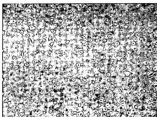
Compound 9
