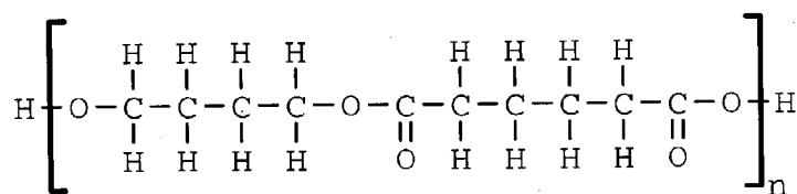
poly(buthyleneglycol adipinat)
