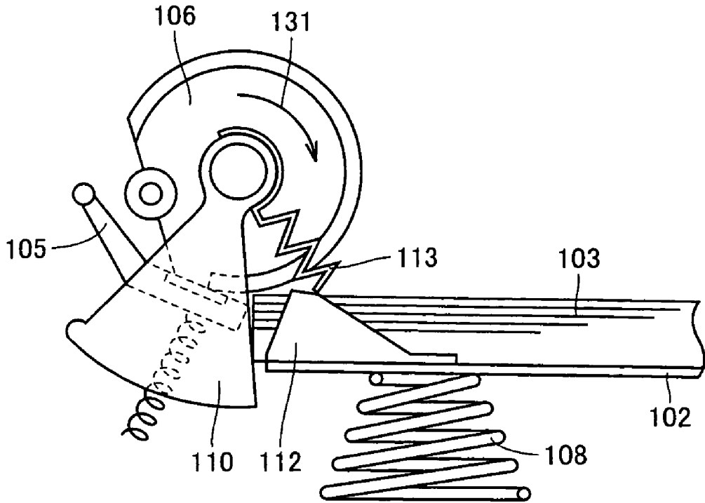
FIG.11 PRIOR ART
