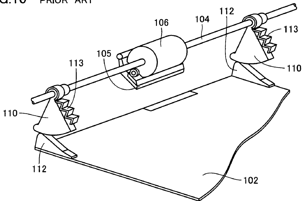
FIG.10 PRIOR ART
