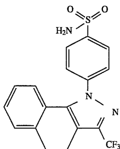
4,5-Dihydro-4-[3-(trifluoromethyl)-1H-benz[g]indazol-1-yl]benzenesulfonamide
