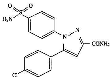
4-[4-(Aminosulfonyl)phenyl]-5-(4-chlorophenyl)-1H-pyrazole-3-carboxamide
