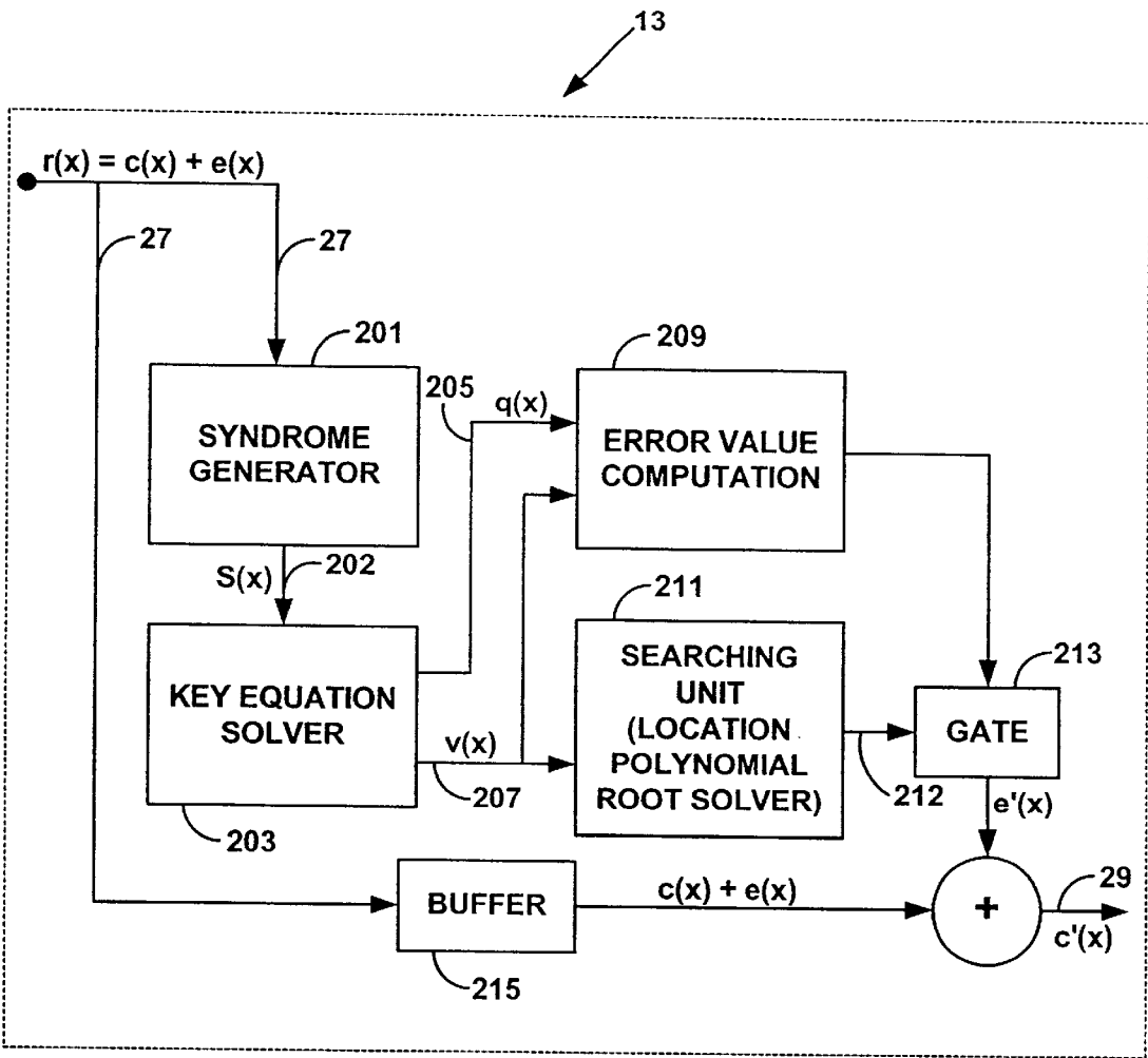
FIG. 2 ECC READ PROCESSOR (PRIOR ART)
