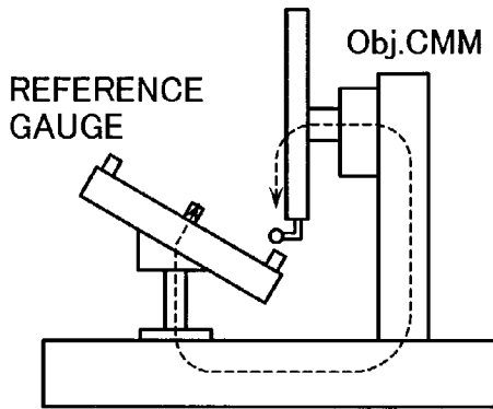
STEP GAUGE
