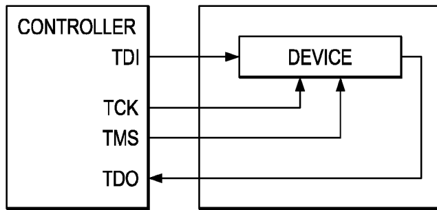
FIG. 4 (PRIOR ART)
