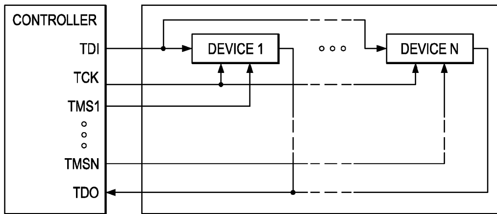
FIG. 5 (PRIOR ART)
