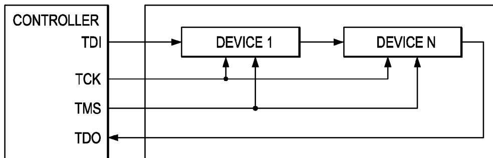
FIG. 6 (PRIOR ART)
