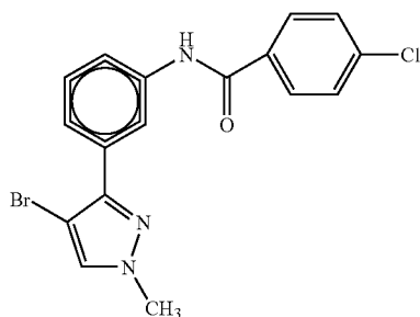
m = 0, R 1 = H, R 4 = chlorophenyl N-[3-(4-bromo-1-methylpyrazol-3-yl)phenyl][4-chlorophenyl]carboxamide
