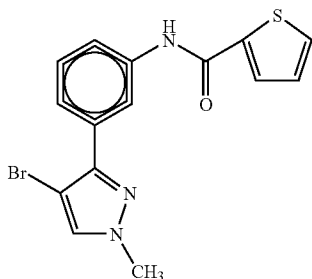
m = 0, R 1 = H, R 4 = thiophene N-[3-(4-bromo-1-methylpyrazol-3-yl)phenyl][2-thienyl]carboxamide
