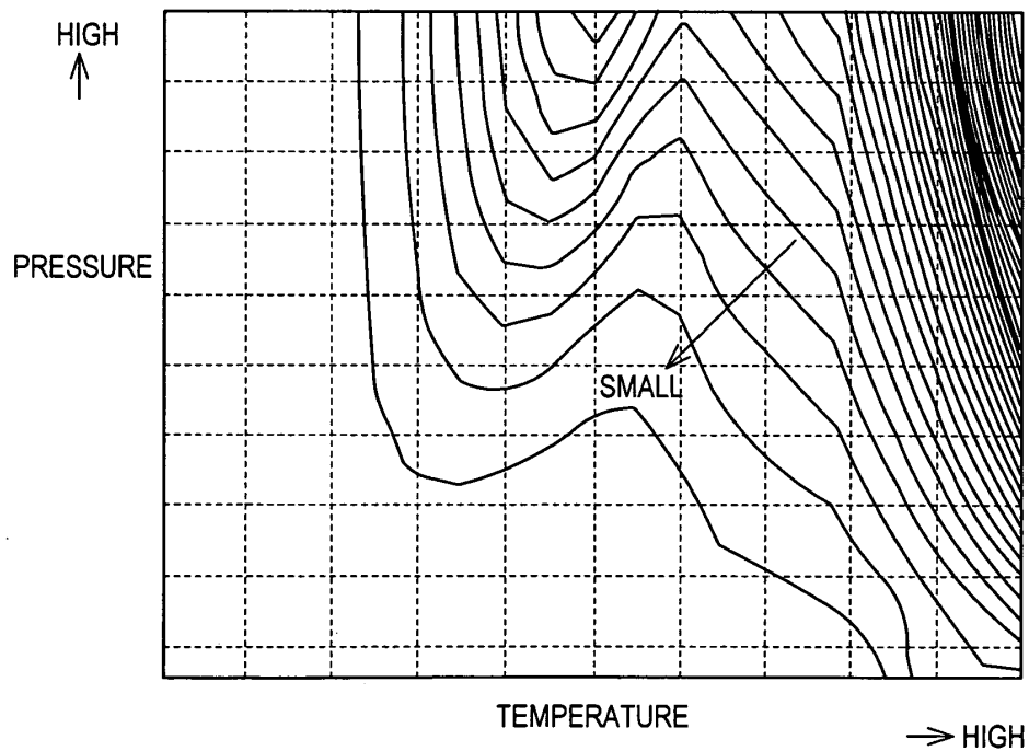
1/τ MAP FOR OCTANE NUMBER 80
