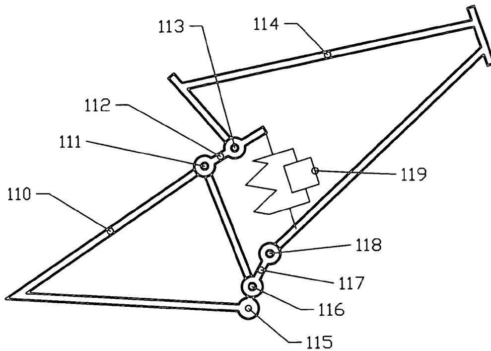
Fig 8 Prior Art
