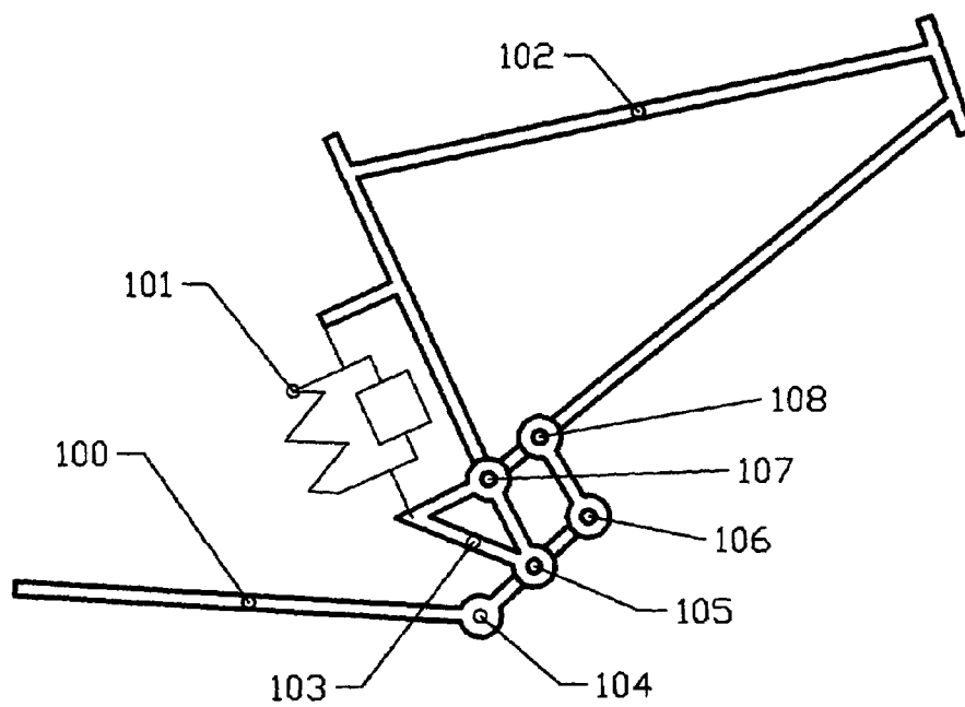
Fig 7 Prior Art
