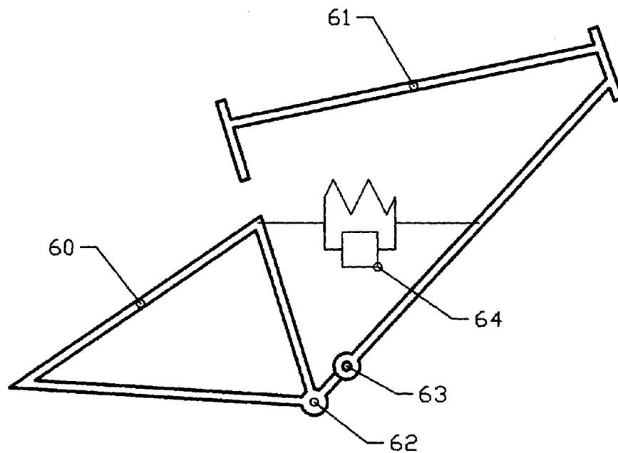
Fig 3 Prior Art
